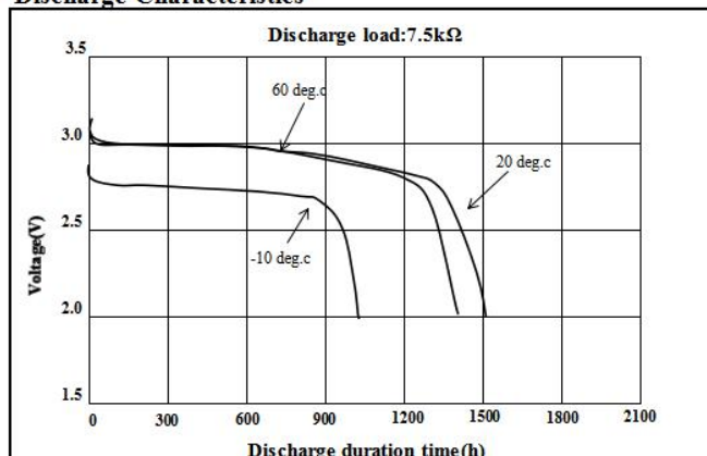
Discharge Characteristics
