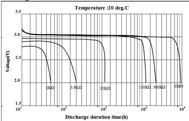
Discharge Characteristics
